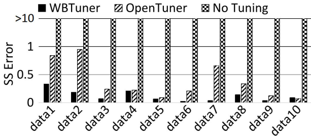
Fig. 15. Phylip tree tuning scores on 10 datasets.
