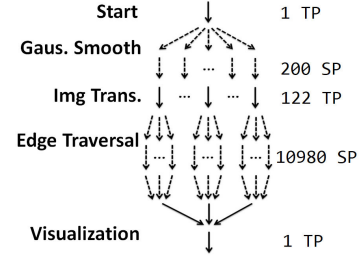
Fig. 6. Tuning Canny. TP/SP are tuning/sampling processes.
