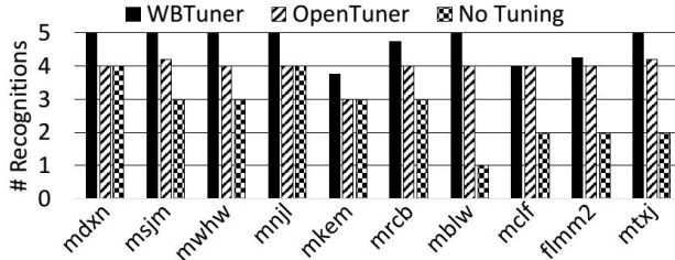
Fig. 20. Sphinx tuning of 10 datasets
