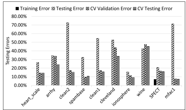
Fig. 17. SVM tuning scores of 10 datasets w/wo validation
