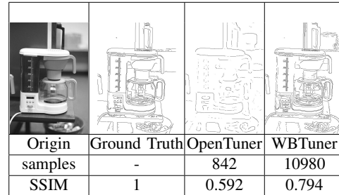
Fig. 7. Tuning Canny with image coffeemaker in 90s.
