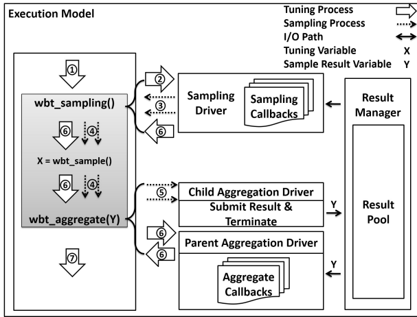
Fig. 5. Execution Model
